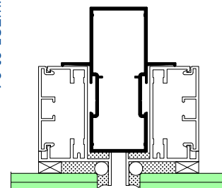
Typical Flush Glazing
