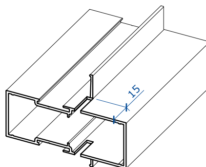
Mullion/Transom
