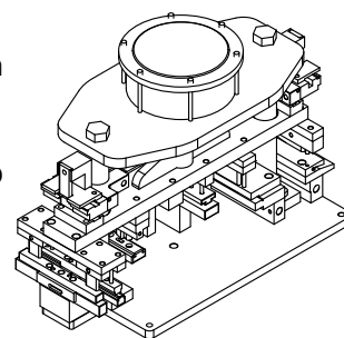
HEX170 pneumatic tool
