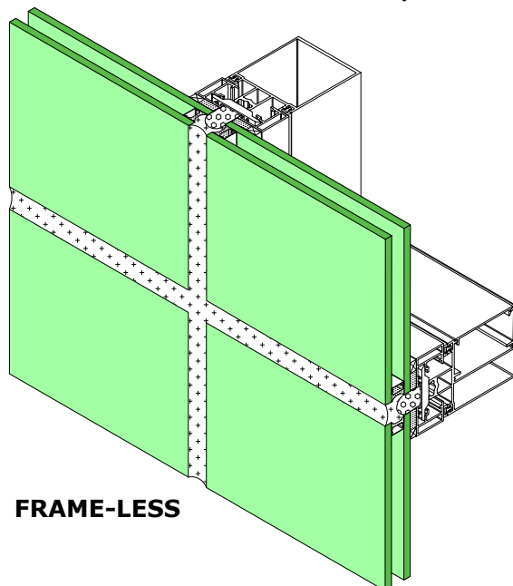
FLUSH GLAZING
